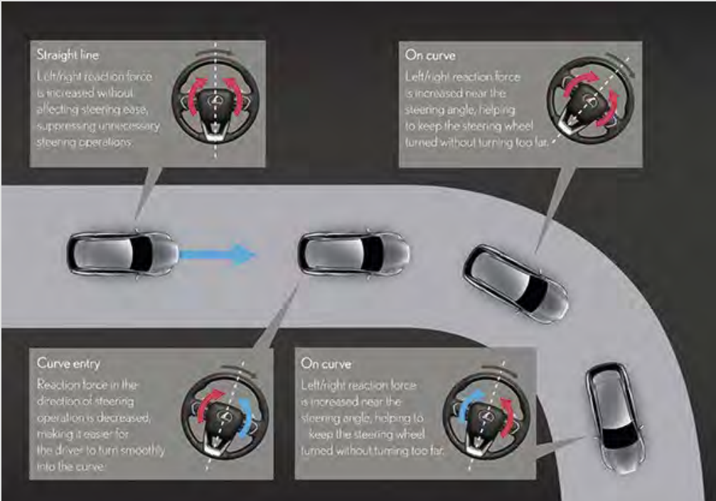
PDA (Steering assist) The system varies steering force in response to differences between the road geometry and driver operation, providing subtle and natural assistance to support smooth steering.
